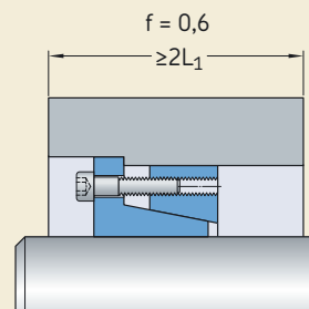
Wider hubs without centering guides, length \geq 2L_1
